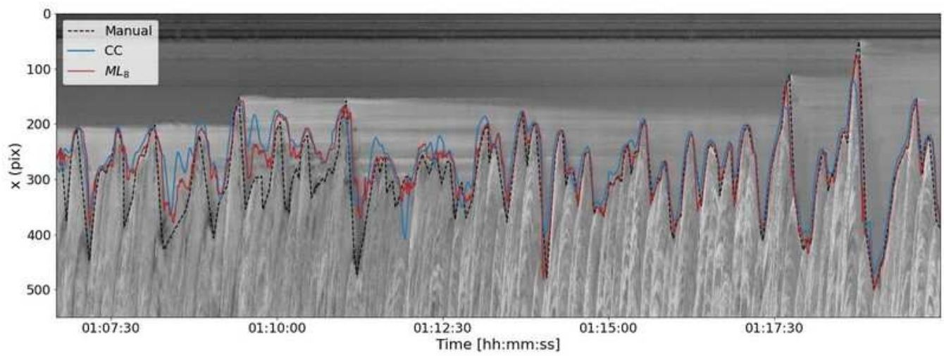
Figure 1: Section timestack from November 14th (video ID: GX050084), with the manually digitized water line (back dashed), and the CC (blue solid) and ML results (red solid).
